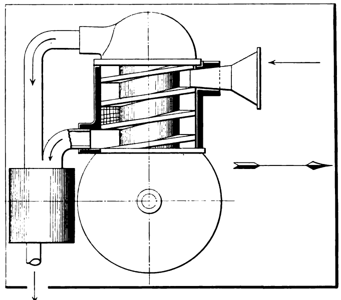
Fig. 58—The exhaust products of combustion are used to whisk the cooling air along
